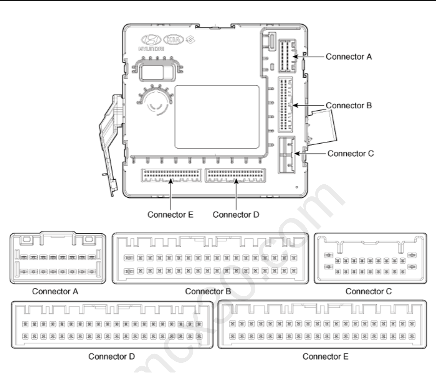
Connector Pin Information
